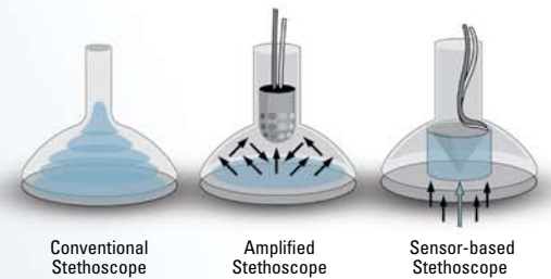
Transducer Placement Elite Electronic's surface placement eliminates sound loss
